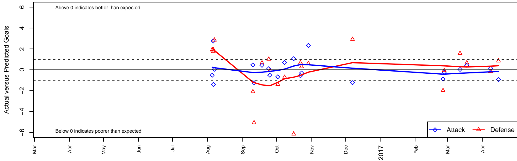
Pelada FA Willamette G03 Dots are actual minus expected GF (blue circles) and GA (red triangles). Blue line is smoothed change in attack strength. Red is smoothed change in defense strength.
